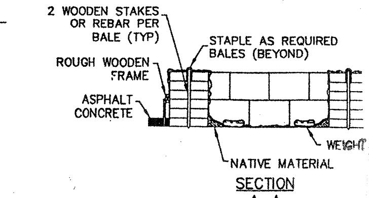
TEMPORARY CONCRETE WASHOUT FACILITY
