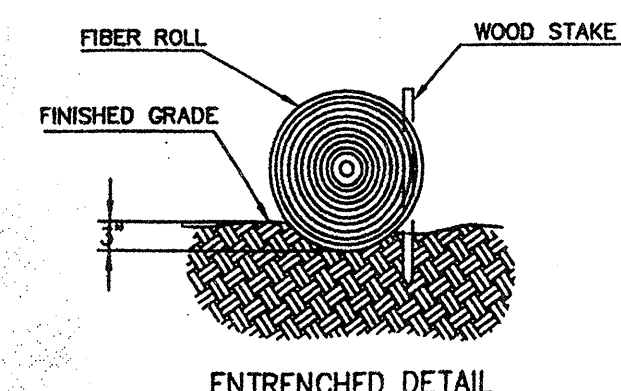
ENTRENCHED DETAIL IN FLAT AREA
