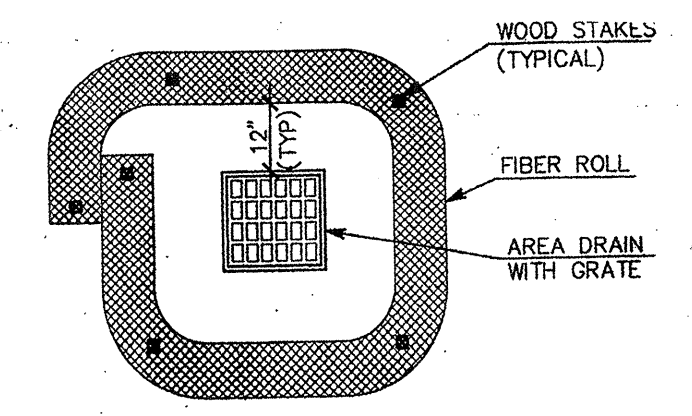
DRAIN INLET PROTECTION DETAIL (NOT TO SCALE)
