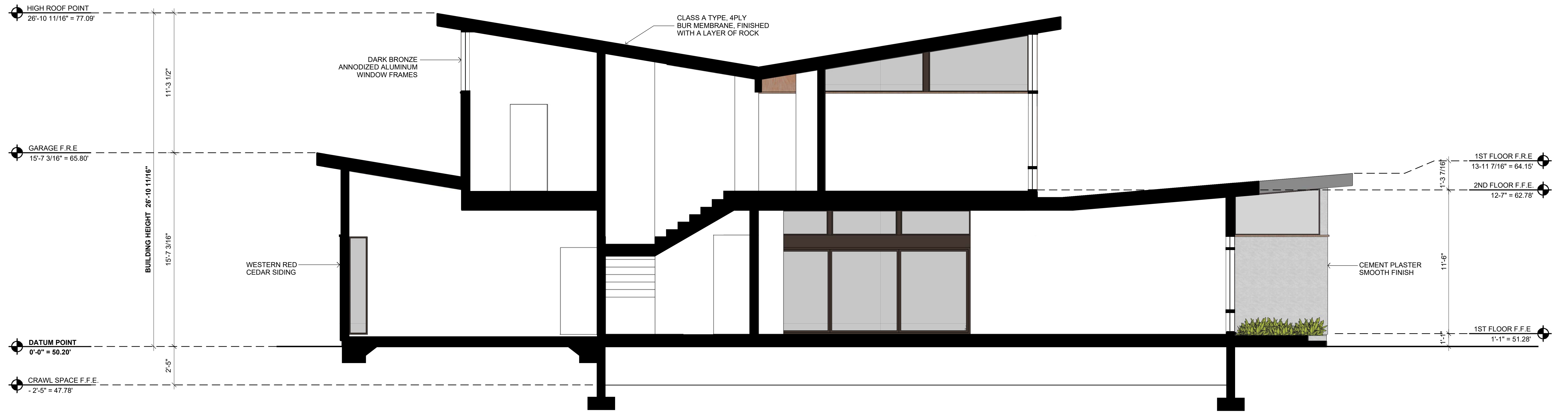
LONG BUILDING SECTION SCALE: 1/4" = 1'-0" 1
