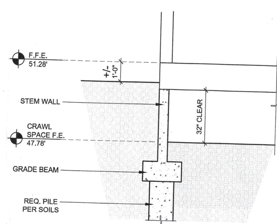
RAISED FOUNDATION DETAIL
