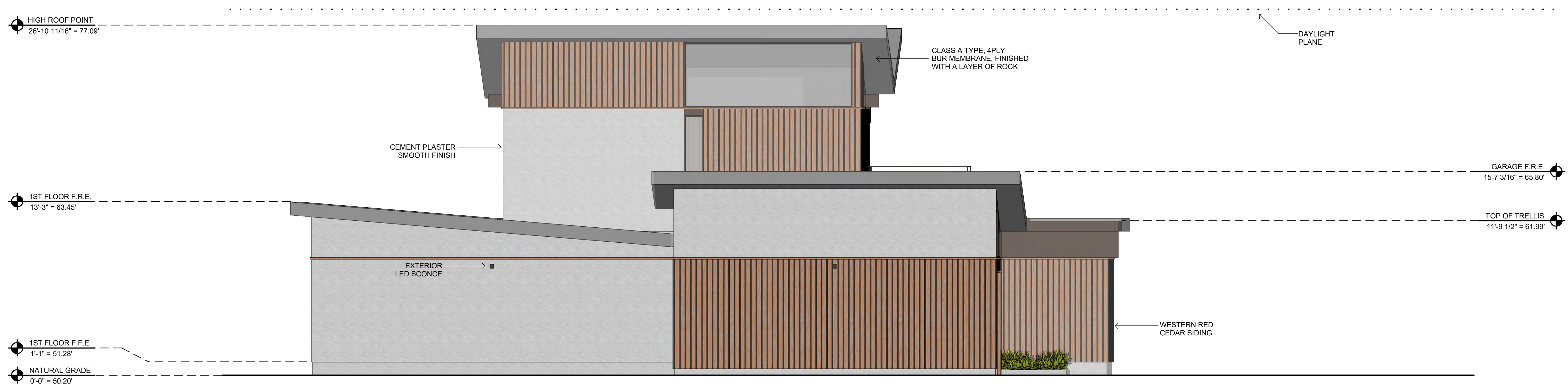
EAST EXTERIOR ELEVATION 2 SCALE: 1/4" = 1'-0"
