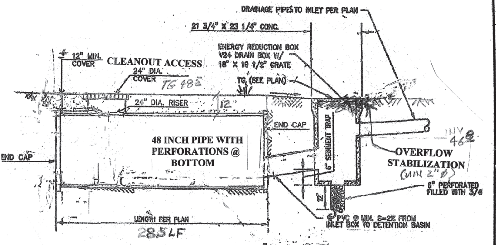
RETENTION PIPE DETAIL (NOT TO SCALE)
