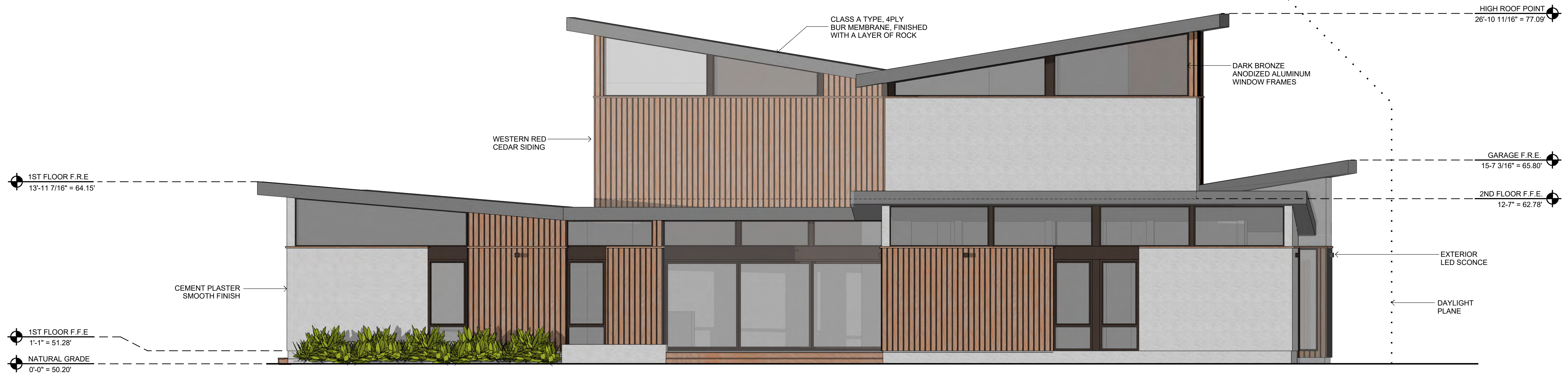
SOUTH EXTERIOR ELEVATION SCALE: 1/4" = 1'-0" 1
